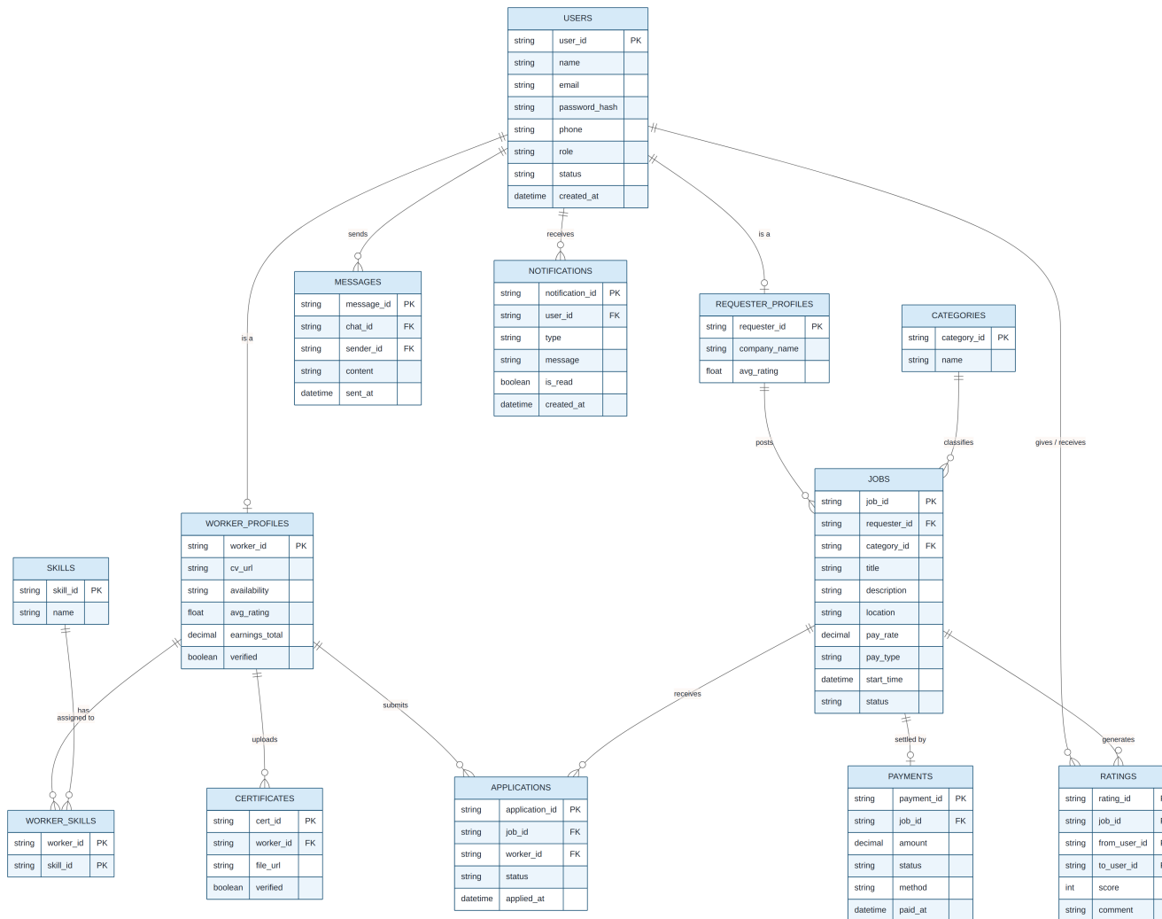
Figure 6 — WorkLink Entity Relationship Diagram
